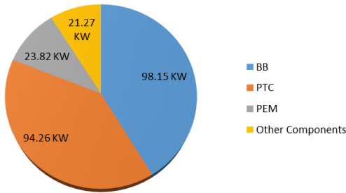
Figure 2. Exergy destruction rates of the components
