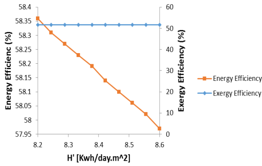
Figure 6. Effect of average daily insolation on horizontal surface on thermal and exergy efficiencies of the quadruple generation system
