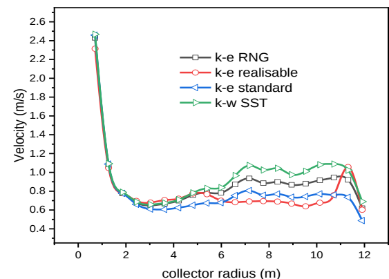
Figure 3. Velocity distribution through collector for the different turbulence models; case zero guides.
