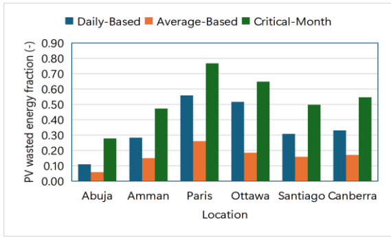
Figure 9. PV wasted energy fraction
