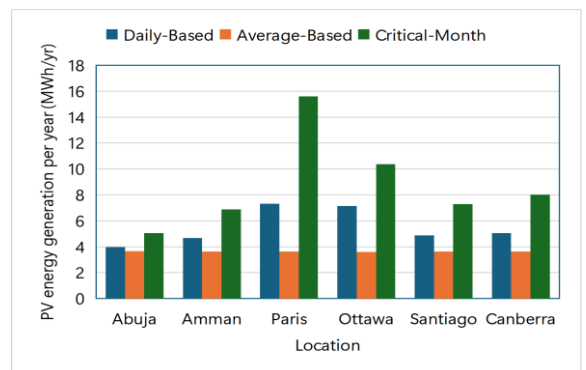
Figure 8. PV energy generation per year
