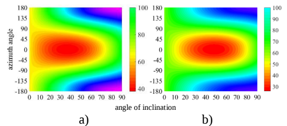
Figure 16. PVS2 orientation-based LCOE ($/MWh), considering the minimum from location-based LCOE for YF-Pp combination in the Best-Case Scenario, for the albedo value: 0.2 (a) and 0.6 (b)
