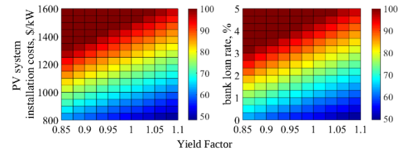
Figure 7. Dependence of the LCOE ($/MWh) of PVS1, on the combined influence of YF, P_p , and F_b in the Worst-Case Scenario
