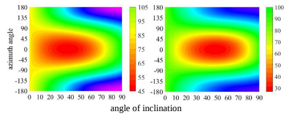
Figure 15. PVS2 orientation-based LCOE ($/MWh), considering the minimum from location-based LCOE for YF-Rb combination in the Best-Case Scenario, for the albedo value: 0.2 (a) and 0.6 (b)
